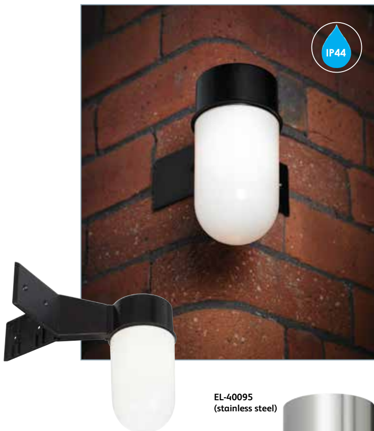
EL-40088 (polycarb corner bracket with glass diffuser)
